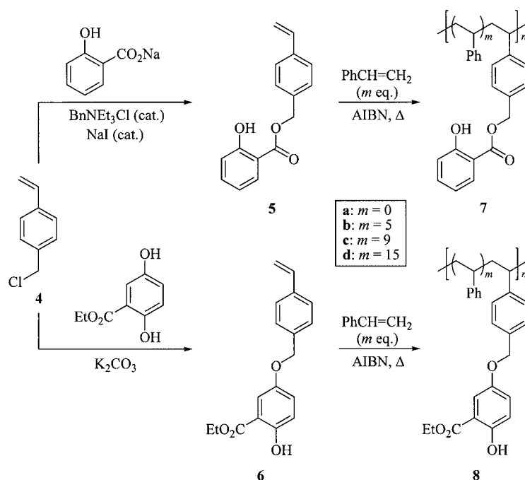
Scheme 2. Synthesis of polymeric proton donors 7 and 8
