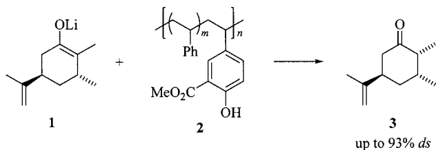
Scheme 1. Diastereoselective protonation of chiral enolate 1 with polymeric, chelating proton donors 2
