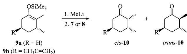
Scheme 3. Diastereoselective protonation of chiral enolates derived from silyl enol ethers 9 with polymeric proton donors 7/8
